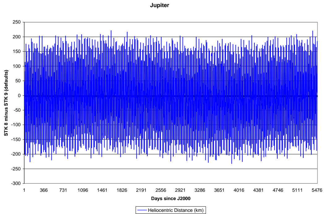
Figure 7. Differences in Reported Jupiter Position (2000-2015)
