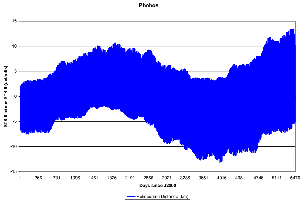
Figure 5. Differences in Reported Phobos Position (2000-2015)
