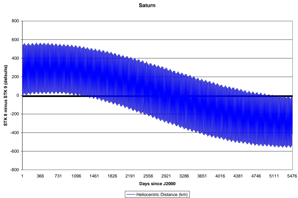
Figure 11. Differences in Reported Saturn Position (2000-2015)
