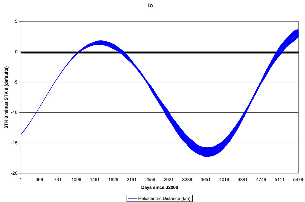
Figure 8. Differences in Reported Io Position (2000-2015)
