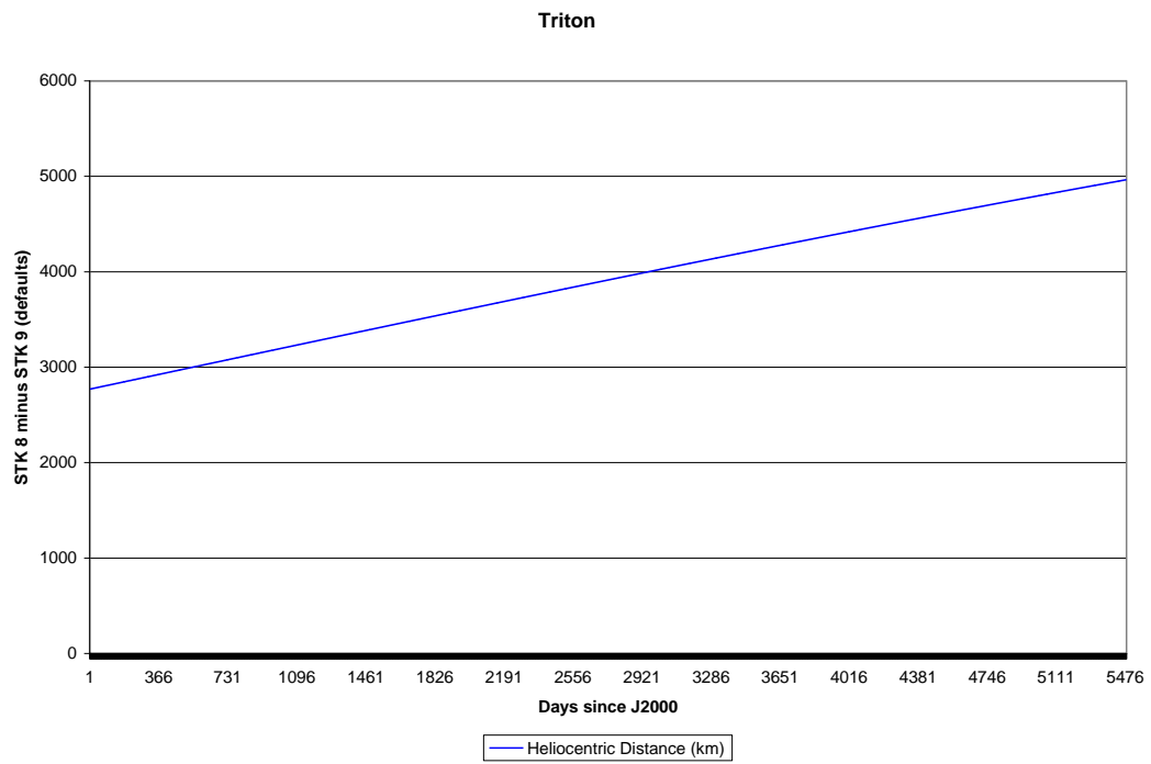
Figure 15. Differences in Reported Triton Position (2000-2015)
