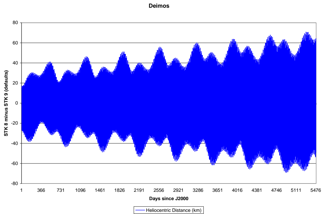
Figure 6. Differences in Reported Deimos Position (2000-2015)
