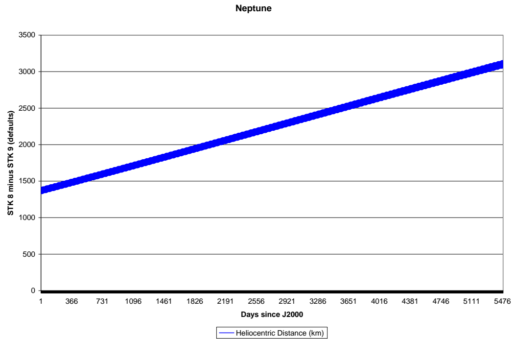
Figure 14. Differences in Reported Neptune Position (2000-2015)
