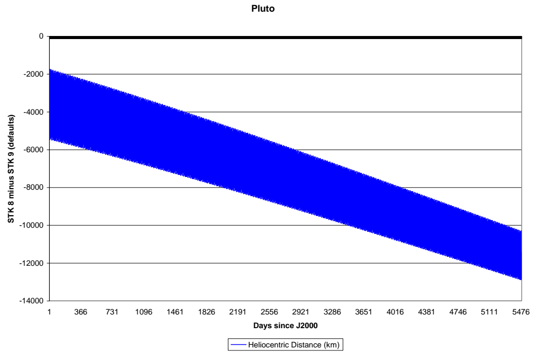
Figure 16. Differences in Reported Pluto Position (2000-2015)
