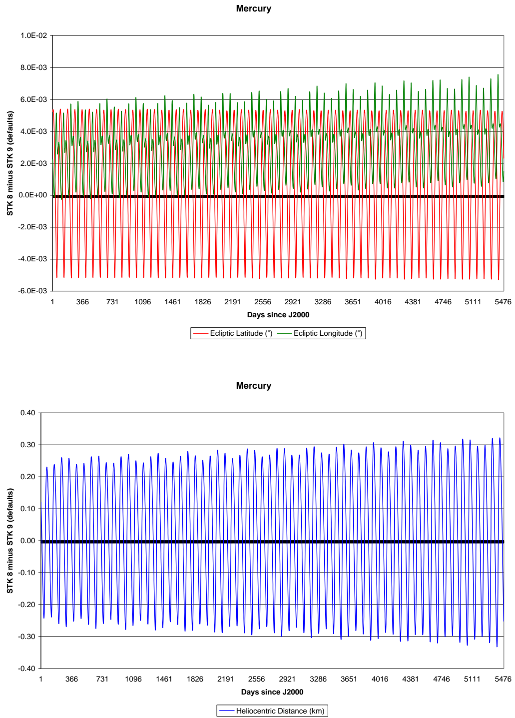
Figure 1. Differences in Reported Mercury Position (2000-2015)
