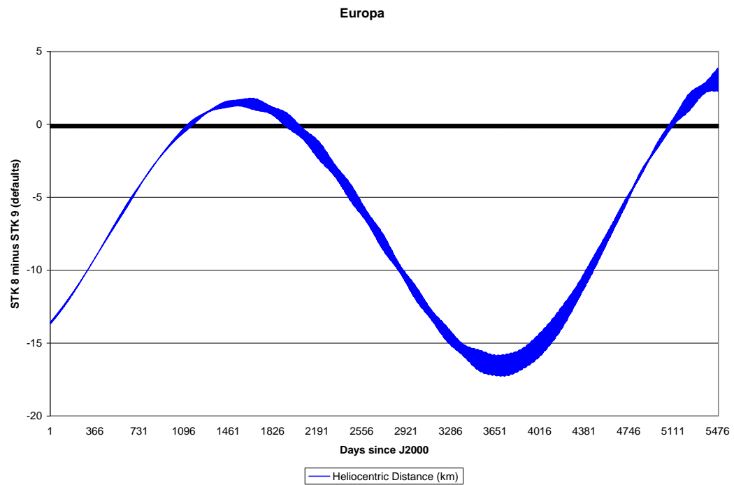
Figure 9. Differences in Reported Europa Position (2000-2015)
