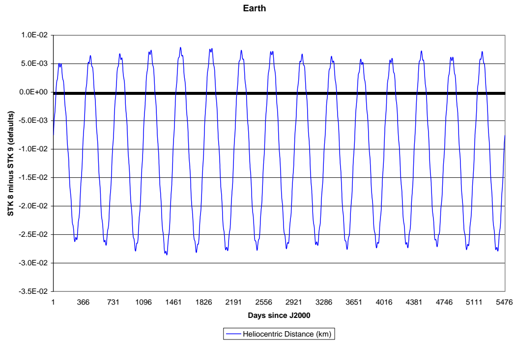
Figure 3. Differences in Reported Earth Position (2000-2015)
