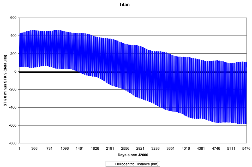
Figure 12. Differences in Reported Titan Position (2000-2015)
