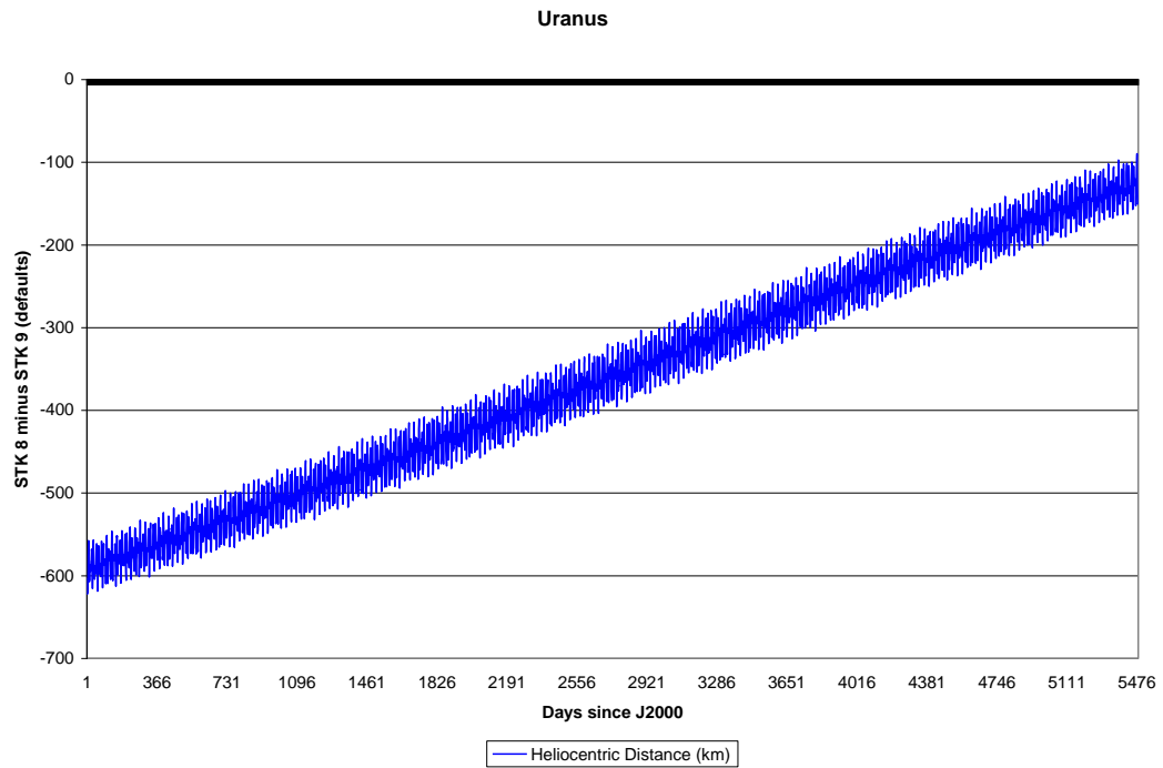
Figure 13. Differences in Reported Uranus Position (2000-2015)
