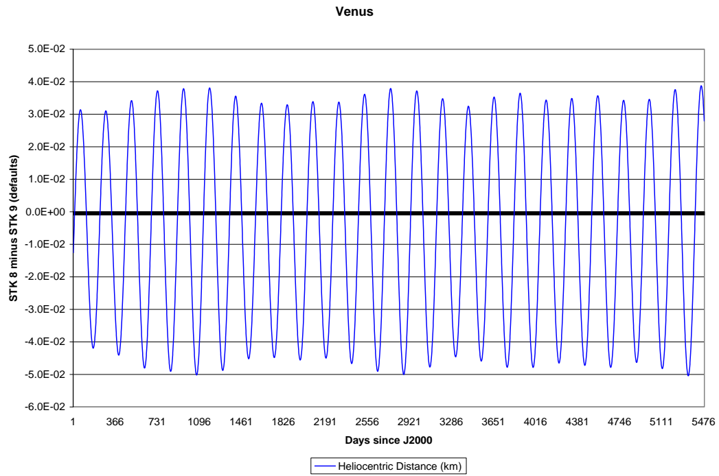
Figure 2. Differences in Reported Venus Position (2000-2015)
