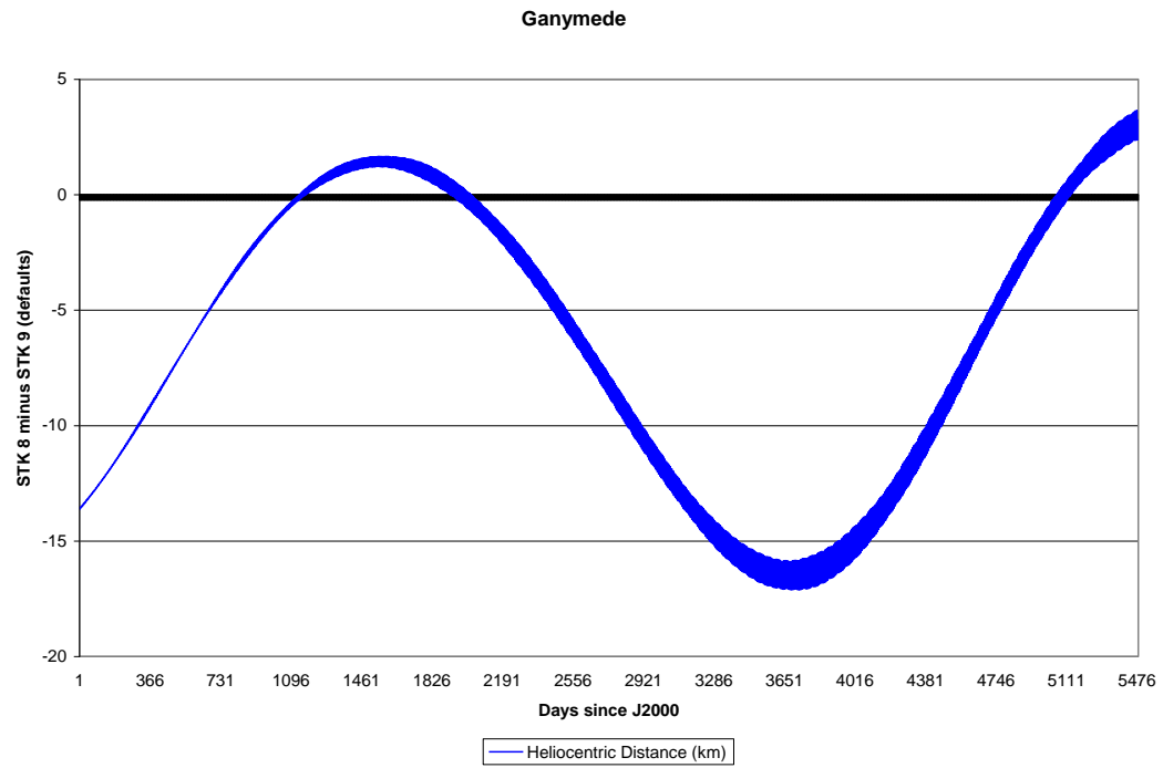
Figure 10. Differences in Reported Ganymede Position (2000-2015)
