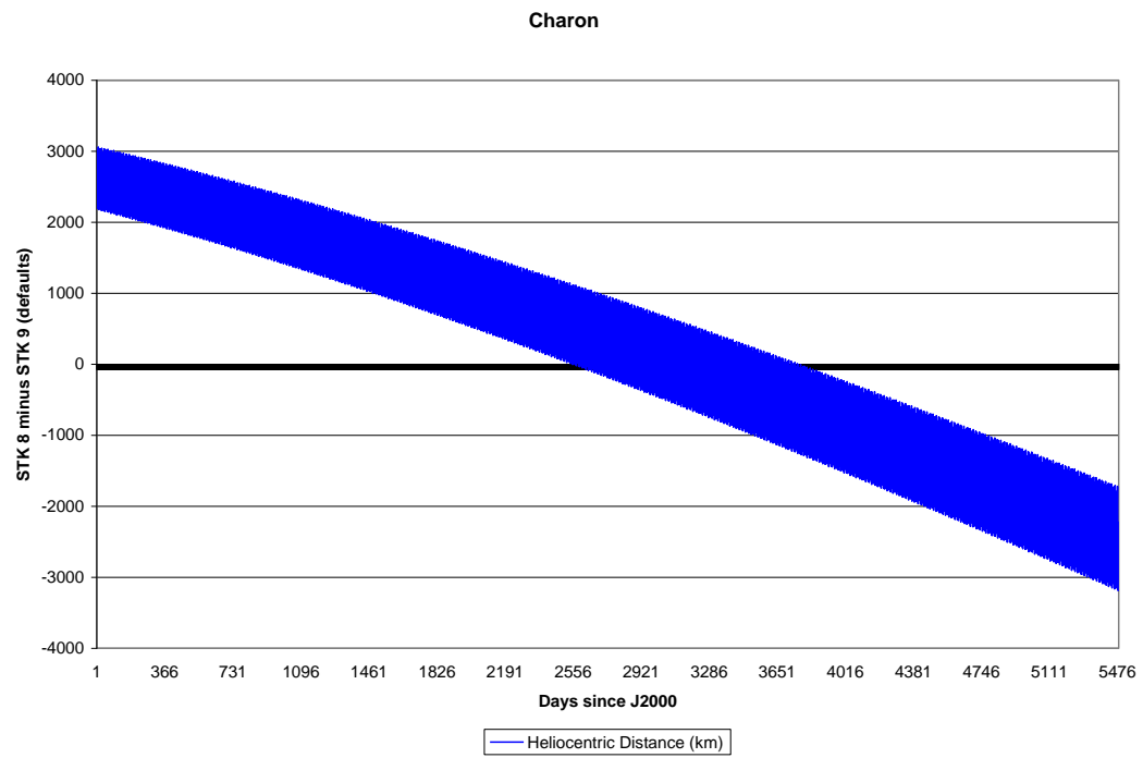
Figure 17. Differences in Reported Charon Position (2000-2015)
