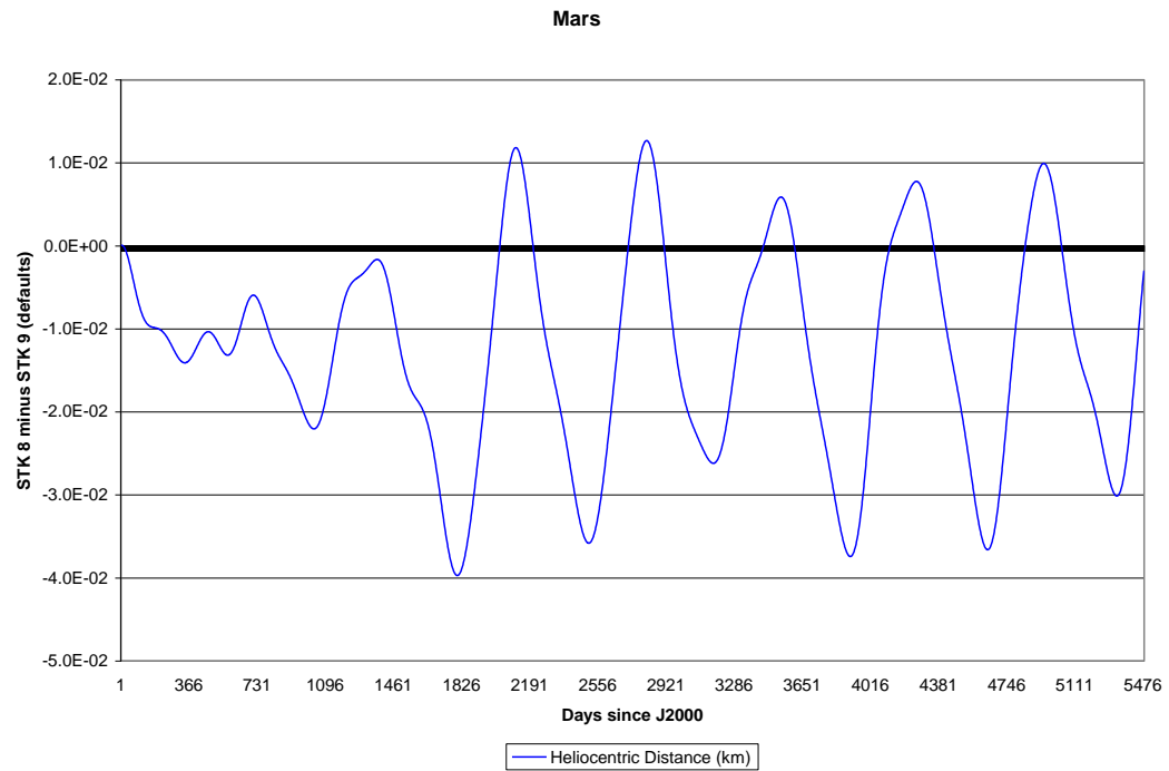
Figure 4. Differences in Reported Mars Position (2000-2015)
