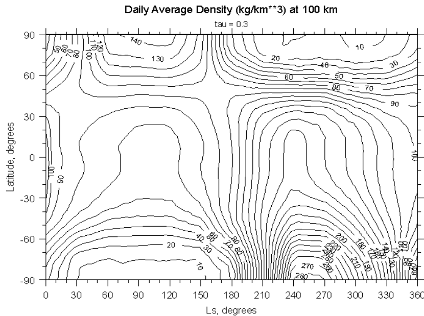
Figure 4.1. Variation of daily average atmospheric density with latitude and season ( L_s angle) at 100 km altitude. Density units are \text{kg/km}^3 . Dust optical depth ( \tau ) is 0.3.
